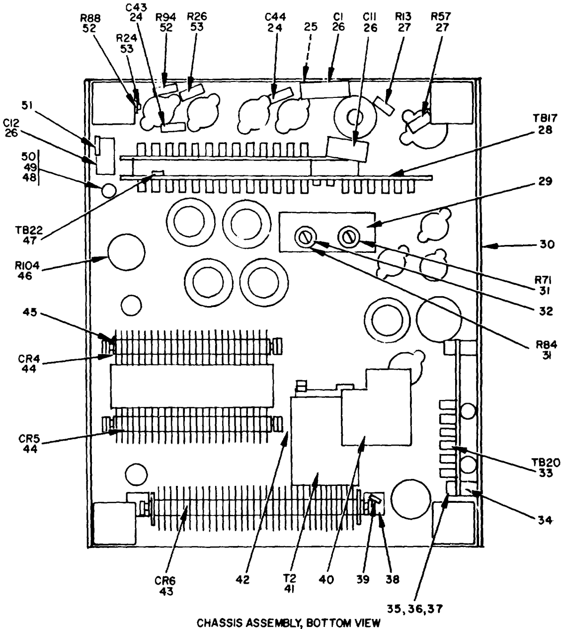
CHASSIS ASSEMBLY, BOTTOM VIEW
